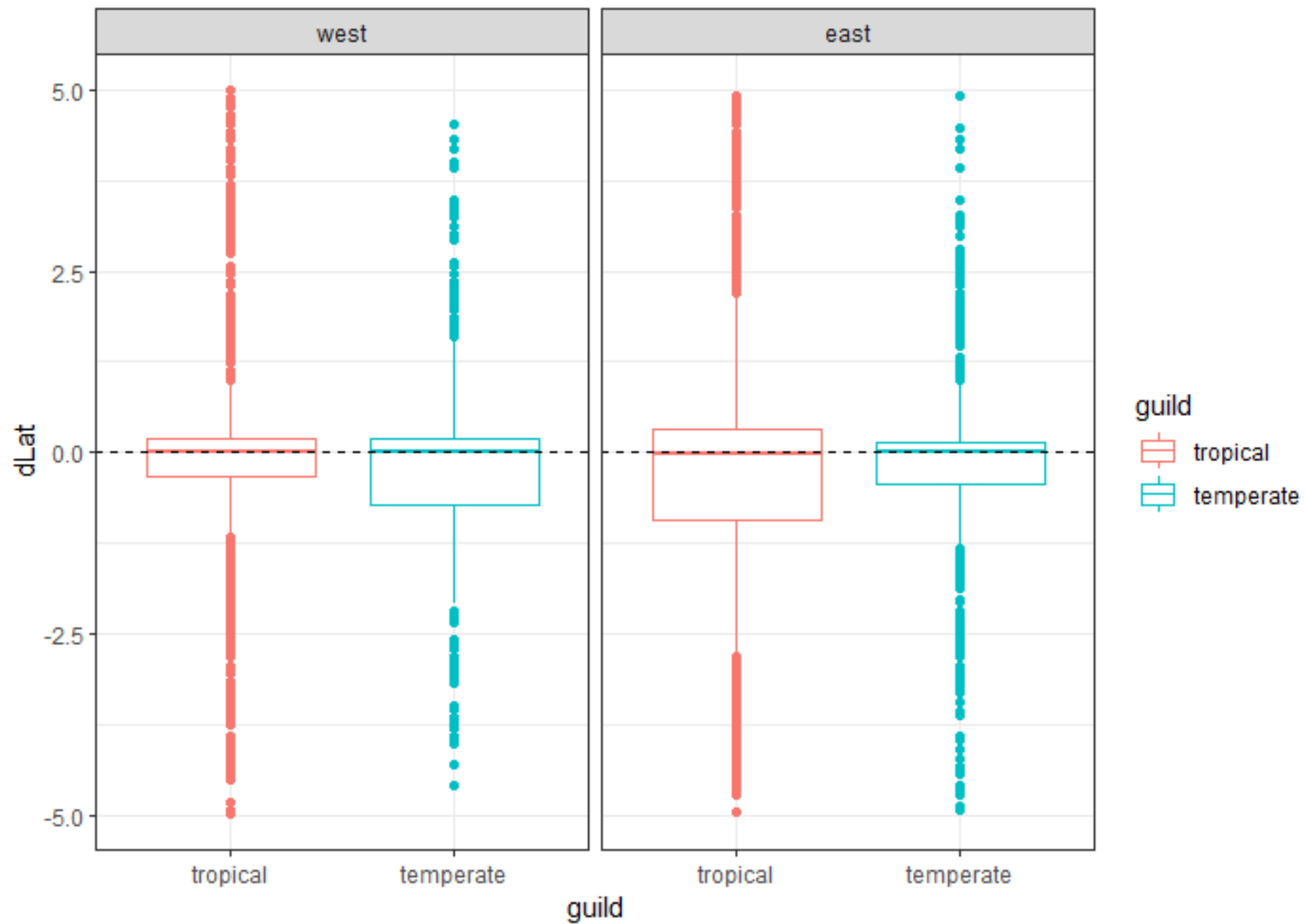
Latitudinal changes before and after 2016 heatwave
