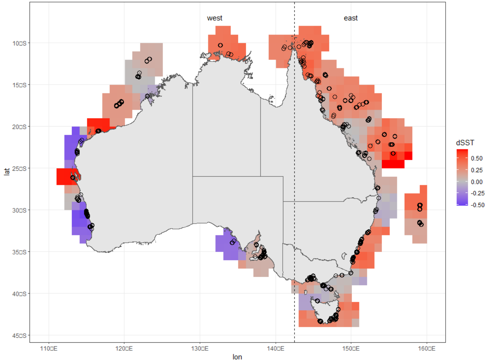
Site distribution and temperature change before and after the 2016 heatwave
